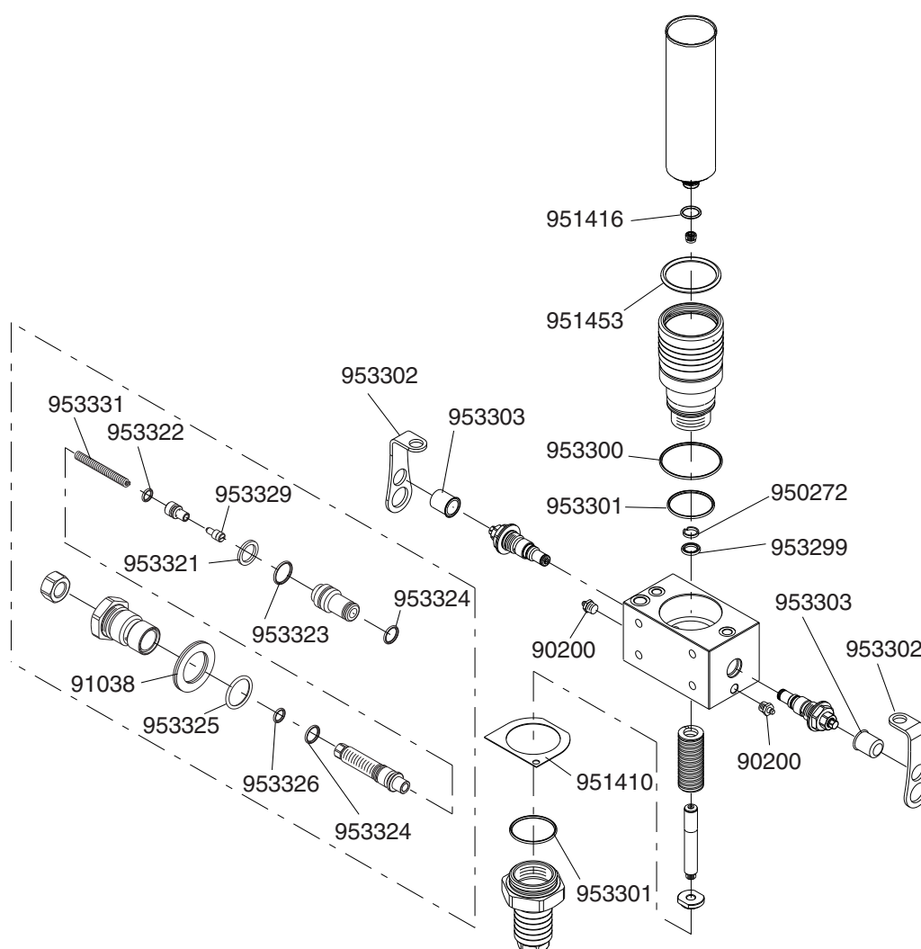
Service kit 953385
